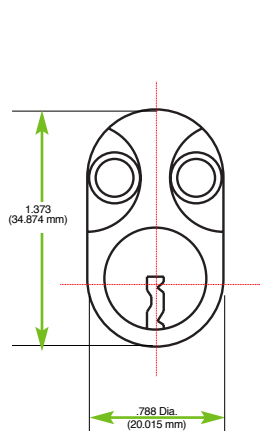
Tailpiece CT-Y76
